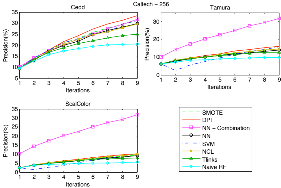
Figure 2: Caltech 256 Dataset - Precision for 9 rounds of relevance feedback.
