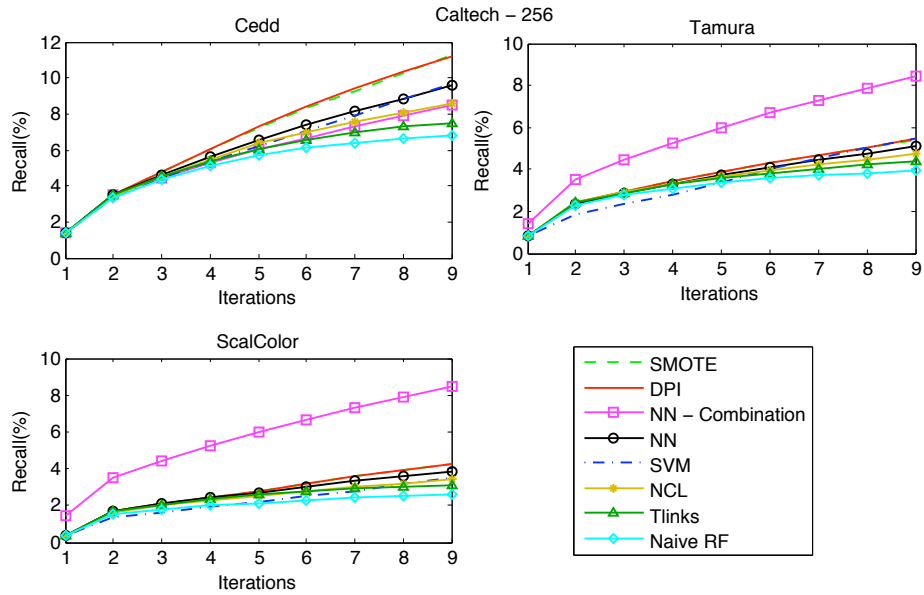
Figure 3: Caltech 256 Dataset - Recall for 9 rounds of relevance feedback.
