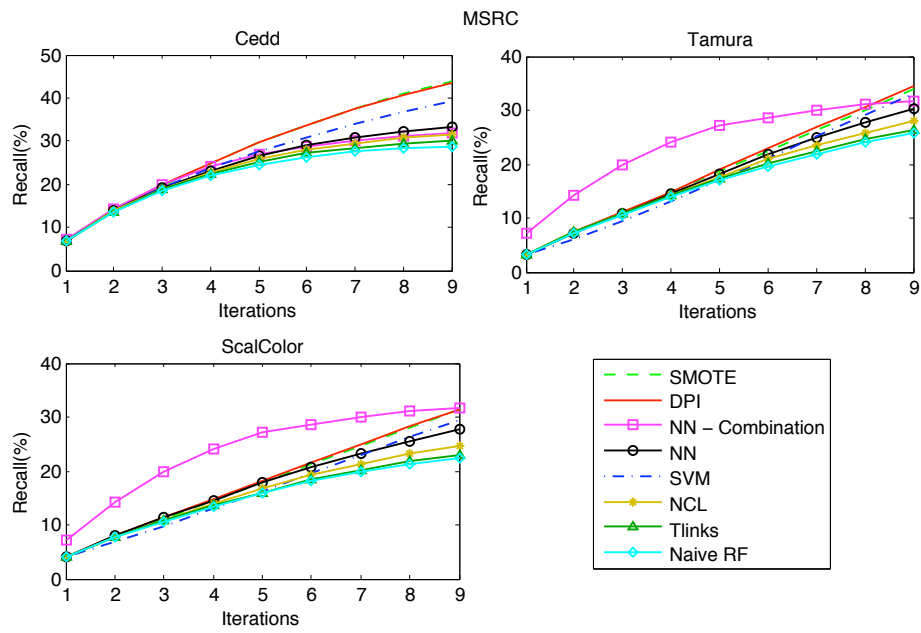
Figure 5: MicroSoft Research Dataset - Recall for 9 rounds of relevance feedback.
