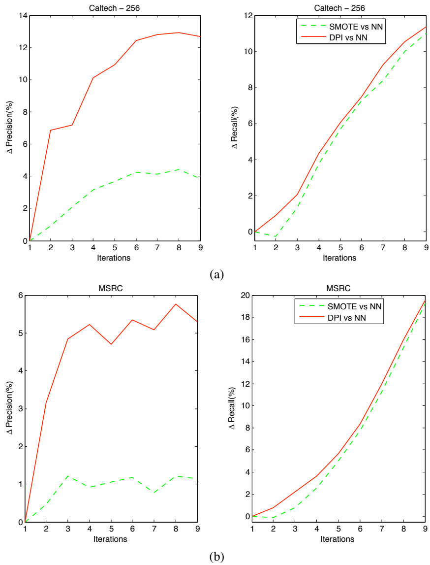
Figure 6: Performance Improvements of SMOTE and DPI against the Nearest-Neighbor technique for relevance feedback, averaged over the three feature spaces. (a) Caltech 256 Dataset - (b) Microsoft Research Dataset
