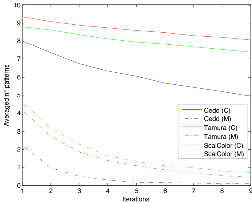
Figure 1: Average number of generated pattern at each iteration.
