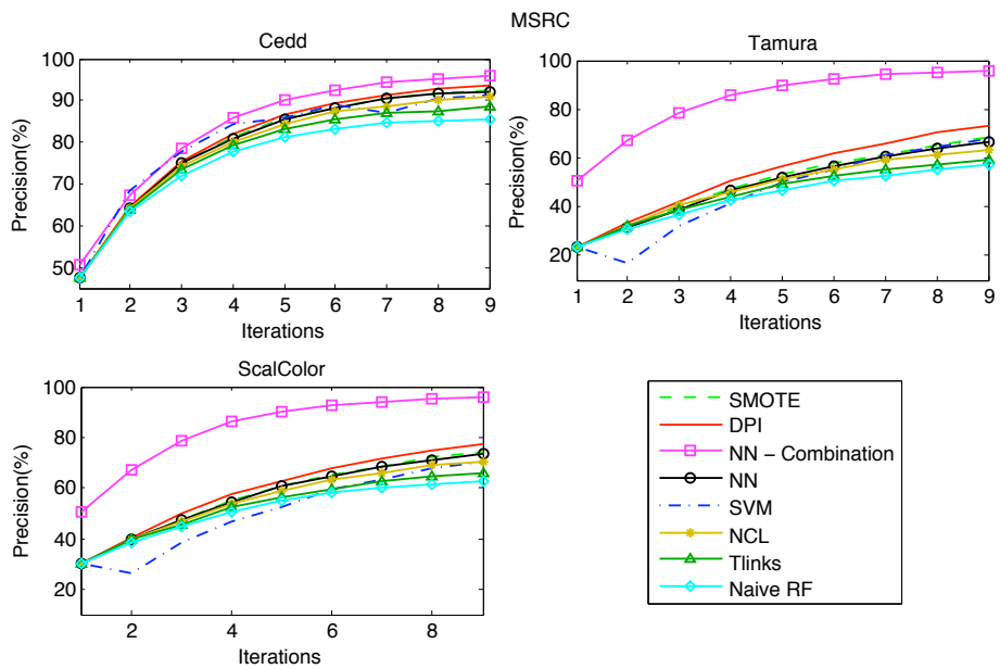
Figure 4: MicroSoft Research Dataset - Precision for 9 rounds of relevance feedback.
